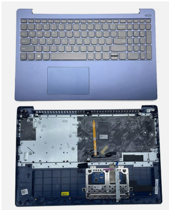
Lenovo Ideapad 330S-15ISK 330S-15IKB palmrest with keyboard
